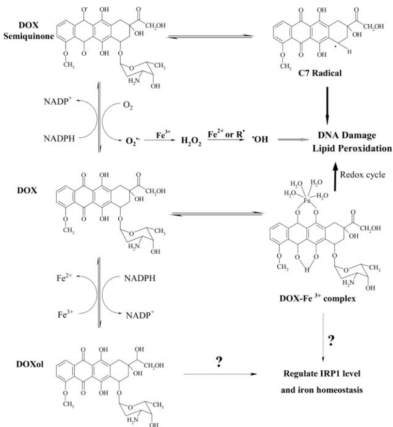
Fig. 4. Illustration of doxorubicin-mediated redox cycling. Doxorubicin can bind to iron by forming doxorubicin-iron(III) complexes, which may lead to ROS formation and cellular damage. One electron reduction of doxorubicin generates the doxorubicin-semiquinone that induces DNA damage and lipid peroxidation by ROS formation. The semiquinone radical can be transformed to a C7 radical that can also mediate cellular damage. The reduction of doxorubicin by two electrons generates a secondary alcohol metabolite, doxorubicinol. Although it is clear that doxorubicin affects cellular IRP1 RNA binding activity and iron homeostasis, it is debatable whether doxorubicinol, the doxorubicin-iron(III) complex, or both are active molecular effectors.
