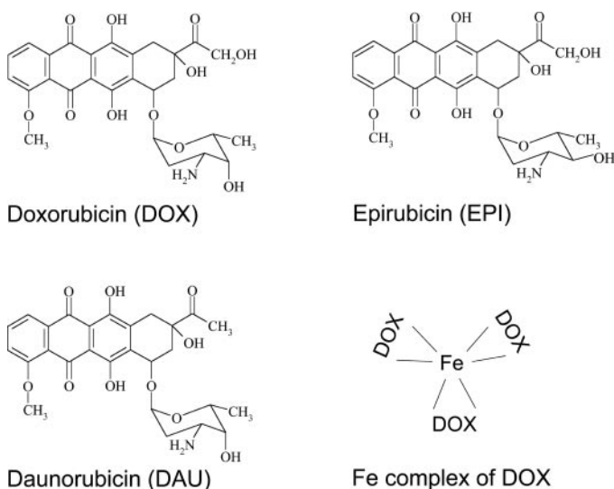
Fig. 1. Illustration of the structures of doxorubicin (Dox), daunorubicin (Daun), epirubicin (Epi), and the iron complex of doxorubicin.
