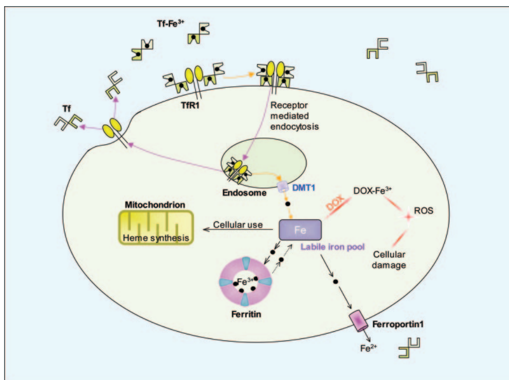
Fig. 2. Schematic illustration of iron metabolism in human cells. Diferric transferrin in the serum avidly binds to TfR1 on the cell membrane. The transferrin-TfR1 complex is then internalized into an endosome by receptor-mediated endocytosis. The iron is released from transferrin by a decrease in endosomal pH that is mediated by a proton pump in the endosome membrane. Once iron is released from transferrin, it is believed to be reduced by a ferrireductase and is then transported through the endosomal membrane by DMT1. Upon leaving the endosome, the iron becomes part of a poorly characterized compartment known as the intracellular labile iron pool. Iron can be redistributed from the labile iron pool for cellular use, stored in ferritin, or potentially pumped out of the cell by ferroportin1. Doxorubicin and other anthracyclines bind iron to form drug-iron(III) complex, which is known to generate ROS and to lead to cellular damage and apoptosis.
