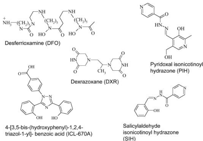
Fig. 7. Illustration of the chemical structures of the iron chelators: desferrioxamine, dexrazoxane, PIH, ICL670A, and SIH.
