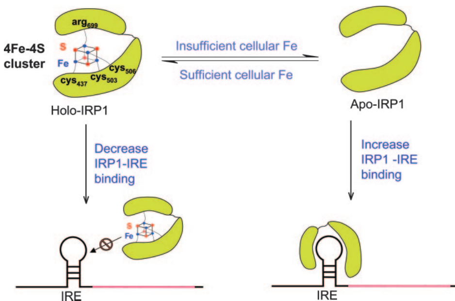
Fig. 3. The mRNA binding activity of IRP1 is regulated by the presence of an [4Fe-4S] cluster within the protein. When cellular iron levels are high, the [4Fe-4S] cluster is present in the IRP1, which abrogates mRNA binding and is known as holo-IRP1 or cytoplasmic aconitase. On the other hand, when cells are iron-depleted, the [4Fe-4S] cluster is absent, and the protein has mRNA binding activity and is known as apo-IRP1.
