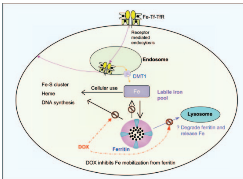
Fig. 6. Schematic illustration of the effect of doxorubicin on cellular iron metabolism. Doxorubicin leads to iron accumulation in ferritin as a result of inhibition of iron mobilization from this protein. There is no change in the total amount of iron in the cell; rather, only the intracellular distribution is markedly affected. The mechanism by which doxorubicin inhibits iron release from ferritin is not known, but may involve, at least in part, disturbance to lysosomal function. Indeed, the lysosome has been reported to be involved in ferritin degradation, and the release of iron from this protein. The inability of ferritin to release iron after exposure to doxorubicin may lead to cytotoxic effects because of the requirement of essential metabolic processes for iron (e.g., DNA synthesis). Clearly, this potential growth-inhibitory mechanism is not the only one mediated by anthracyclines.
