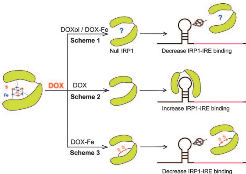
Fig. 5. Proposed mechanisms of action of doxorubicin on IRP1-RNA binding activity. There are three main hypotheses of how doxorubicin regulates cellular IRP1 levels. Scheme 1, doxorubicinol, a secondary alcohol metabolite of doxorubicin, together with cis -aconitate, may act to remove iron from the [4Fe-4S] cluster of holo-IRP1. The removal of iron from the cluster results in the oxidation of doxorubicinol to doxorubicin and generation of the doxorubicin-iron complex, which irreversibly converts IRP1 to a null protein (Minotti et al., 1998). Scheme 2, doxorubicin removes the [4Fe-4S] cluster of holo-IRP1 and increases IRP-IRE binding (Minotti et al., 2001; Kotamraju et al., 2002). Scheme 3, the doxorubicin-iron complex catalyzes disulfide bridge formation between crucial IRP1 thiol groups inhibiting IRP-IRE binding (Kwok and Richardson, 2002).
